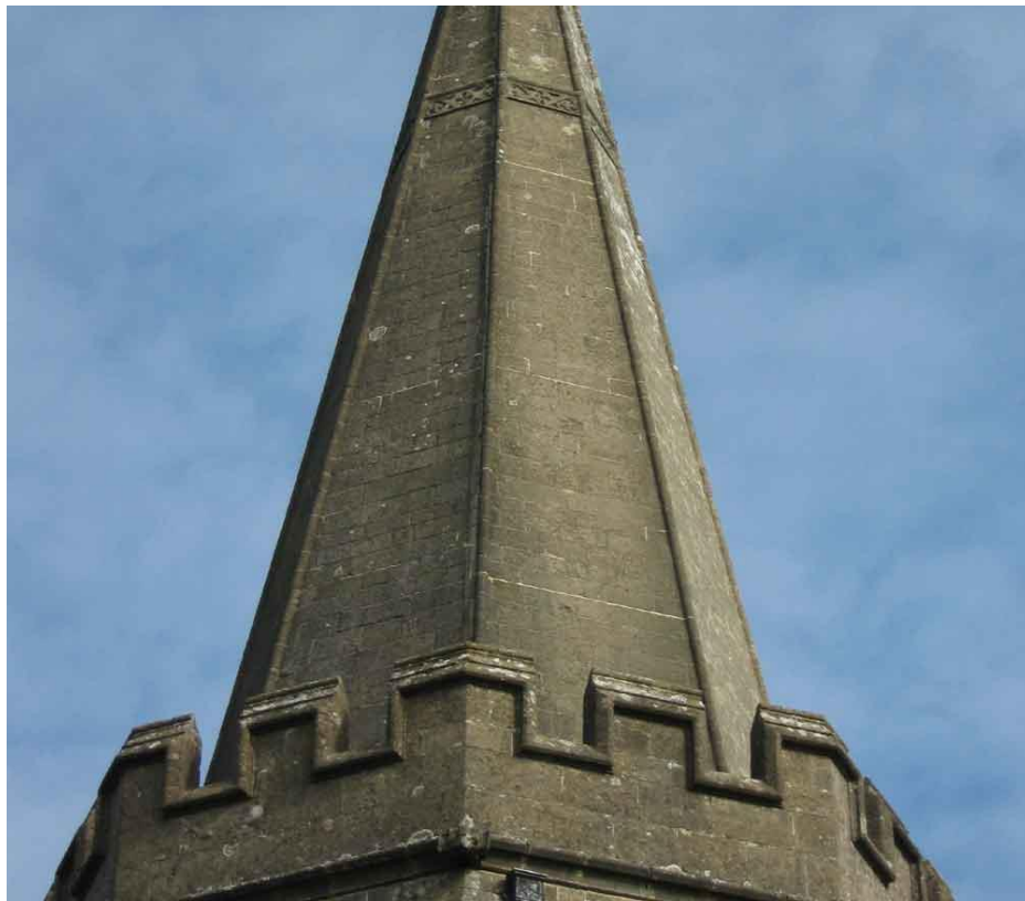
Figure 6 Expansion and re-pointing of the joints associated with ongoing corrosion of three ring beams, St Aldhelms church tower, Doulling.
